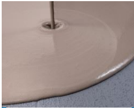
Application of self-levelling smoothing compound on dry Eco Prim Grip Plus on old floor
